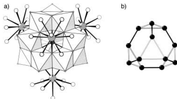
Figure 1. a) Polyhedral representation of the \epsilon -Keggin core in 1 capped with four {La(H 2 O) 4 } 3+ groups. Six of the terminal oxygen atoms of the water molecules on the La 3+ ions have half occupancy factors; b) disposition of the twelve Mo atoms, the Mo–Mo pairs are linked in black.
