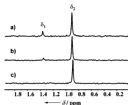
Figure 2. 31 P NMR spectra of an aqueous solution of [ε-PMo 12 O 36 (OH) 4 {La(H 2 O) 4 } 5 ] 5+ (ε-PMo 12 ) to which LaCl 3 was added; the ratios of initial concentrations were a) [La 3+ ]:[ε-PMo 12 ] 0 = 0:1, b) [La 3+ ]:[ε-PMo 12 ] 0 = 0.3:1, c) [La 3+ ]:[ε-PMo 12 ] 0 = 0.8:1.
